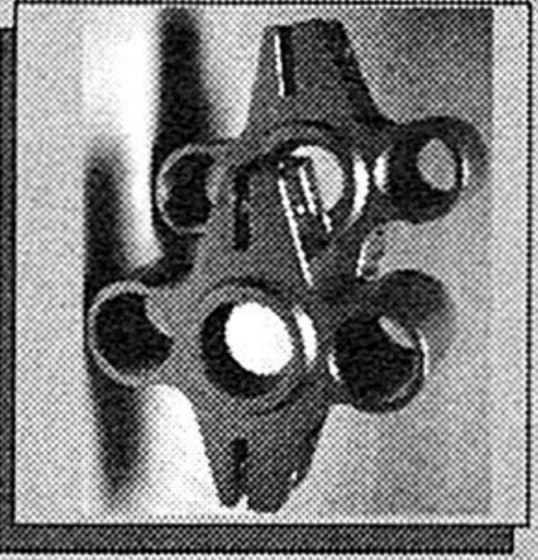
TJR 31 BMT Front Uprights
